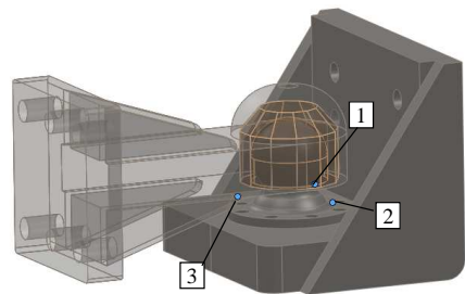
Fig. 7. Three optional points for dynamic analysis
