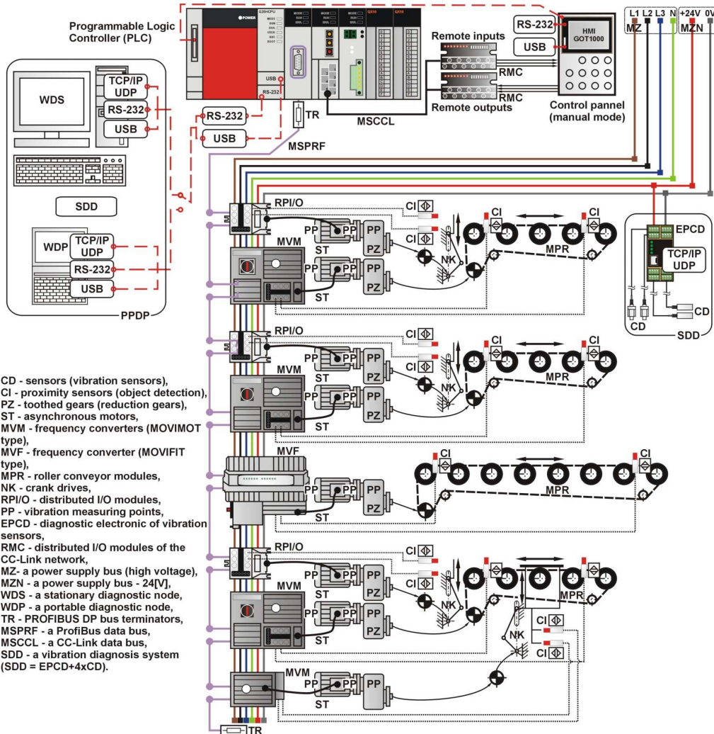
Fig. 1. Schematic view of the laboratory stand
