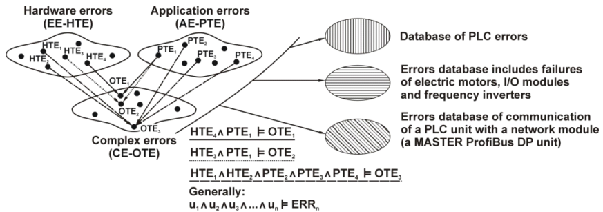
Fig. 3. A manner of definition of complex error implication (CE-OTE type), where: AE-PTE_n , EE-HTE_n \subset u , u – diagnostic premises ( AE-PTE_n or EE-HTE_n , n < N ), ERR_n – logical implication of conjunction of u premises
