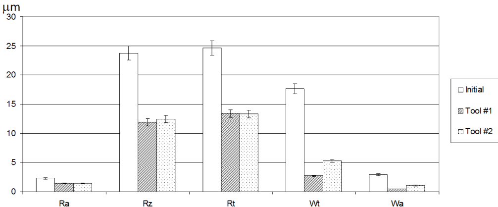
Fig. 11. Average surface roughness and waviness parameters achieved after grinding experiments
