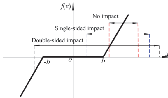
Fig. 2. Nonlinear displacement function
